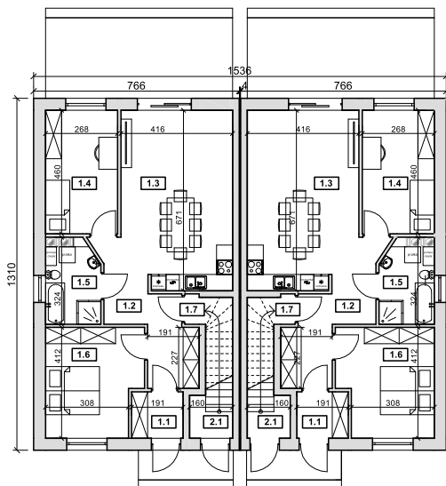
Parter
